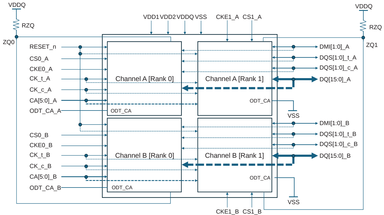
Figure 3.1 – Dual-channel (x32), Dual-rank Package Diagram
