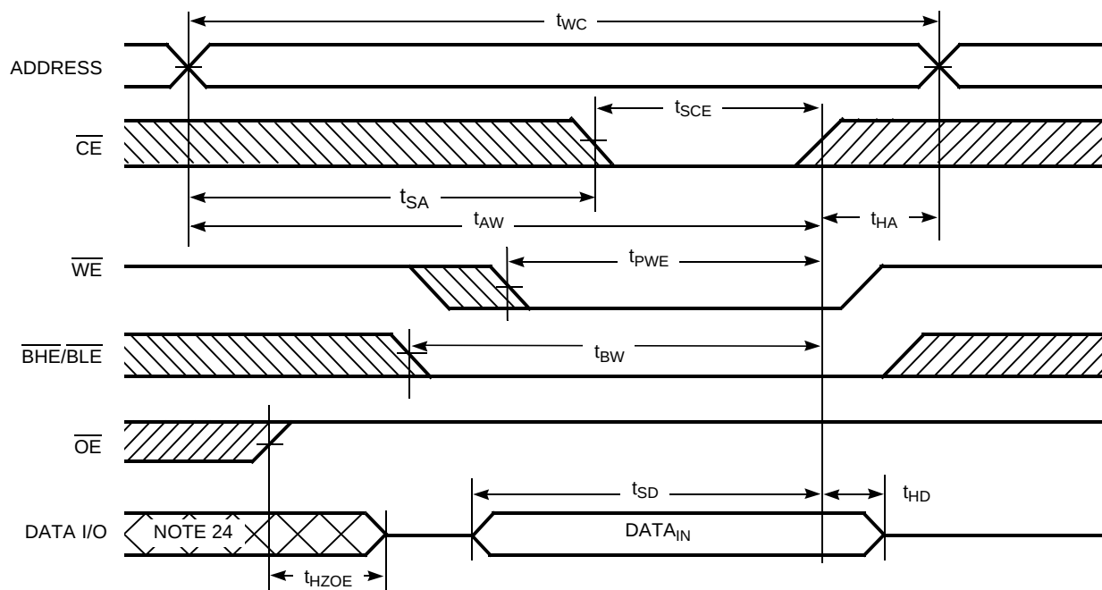
Figure 7. Write Cycle 2: \overline{\text{CE}} Controlled [21, 22, 23]
