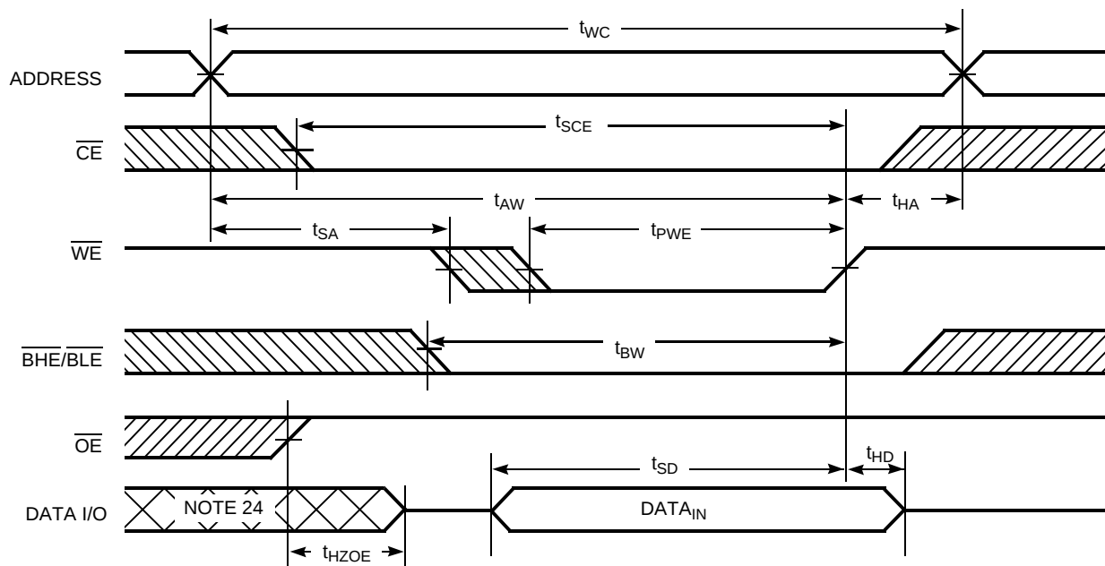
Figure 7. Write Cycle 2: \overline{\text{CE}} Controlled [21, 22, 23]
