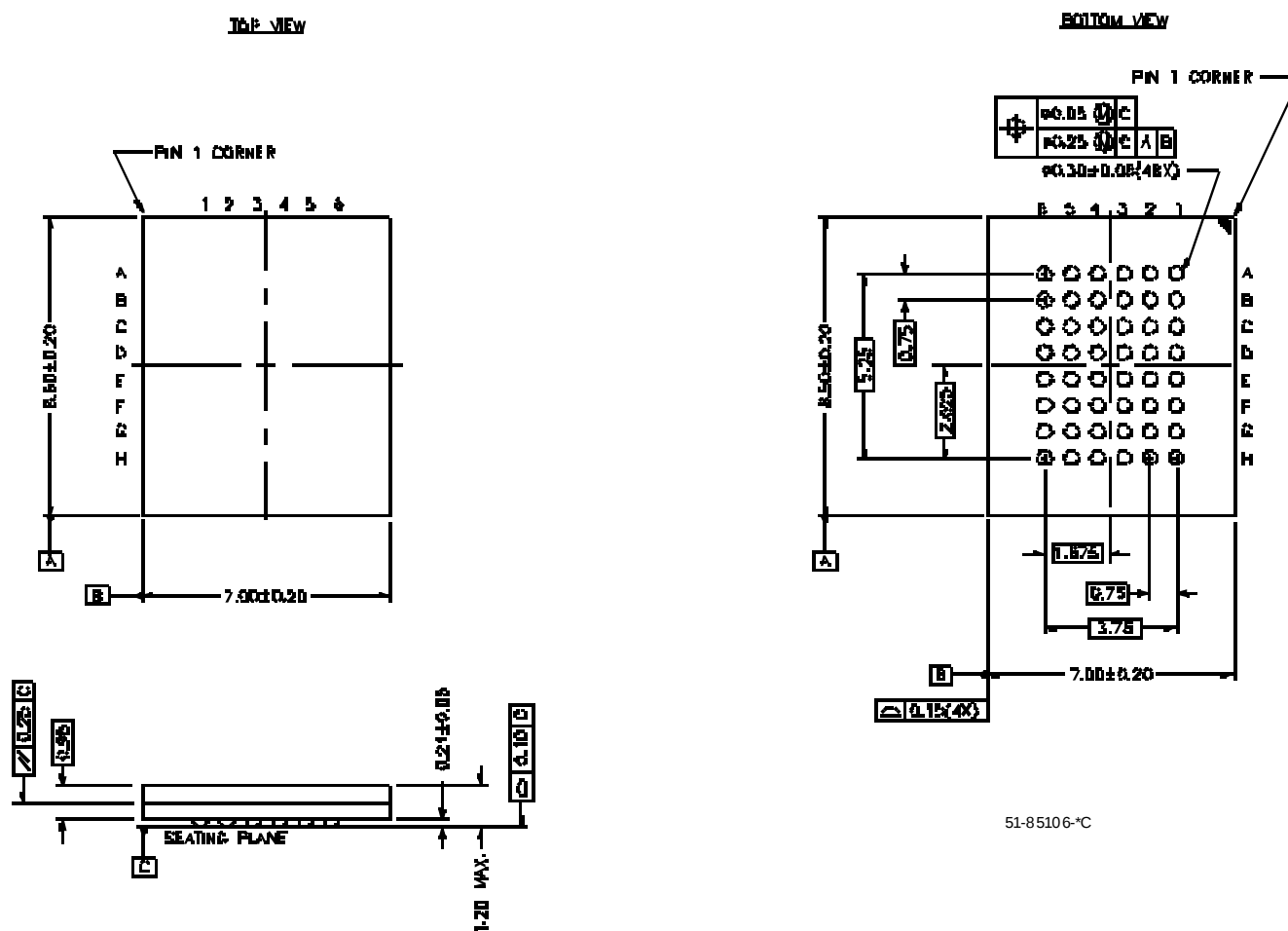
48-Ball (7.00 mm x 8.5 mm x 1.2 mm) Thin BGA BA48B
