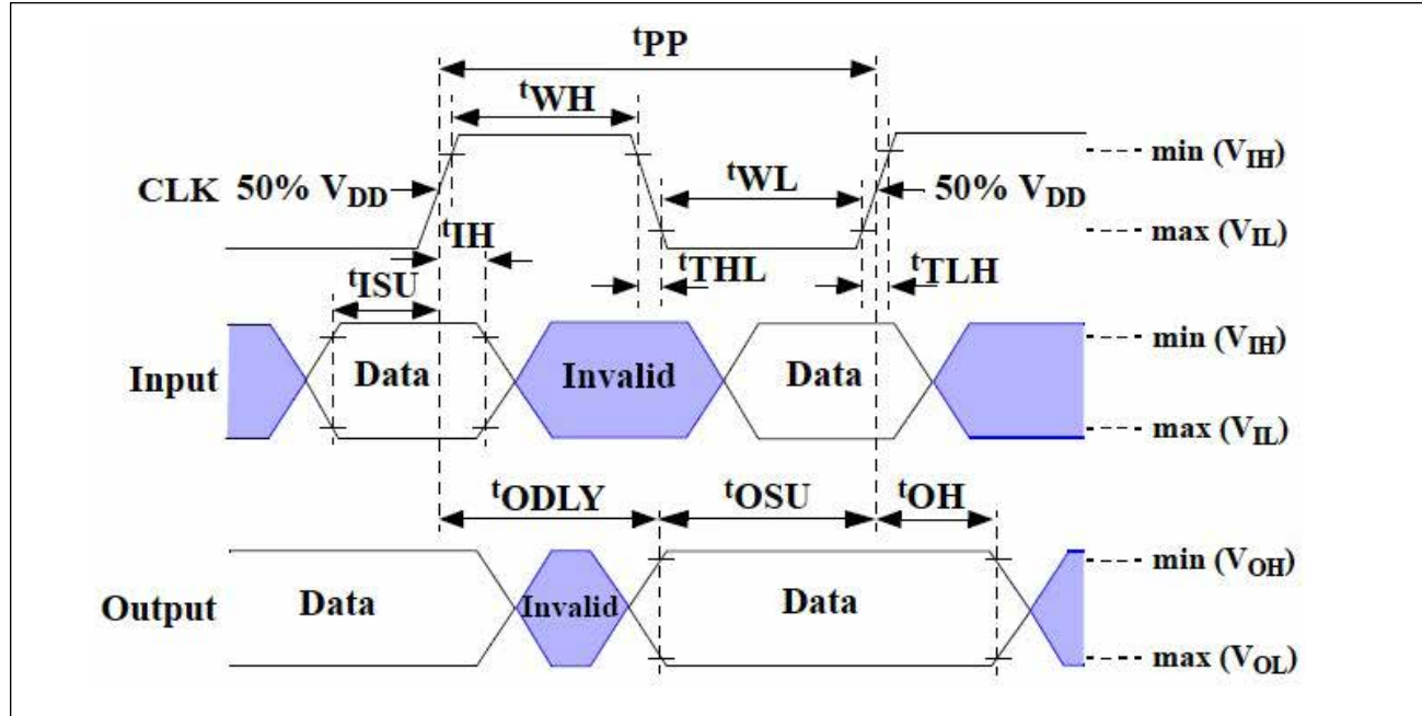
Figure 4. Bus Timing
