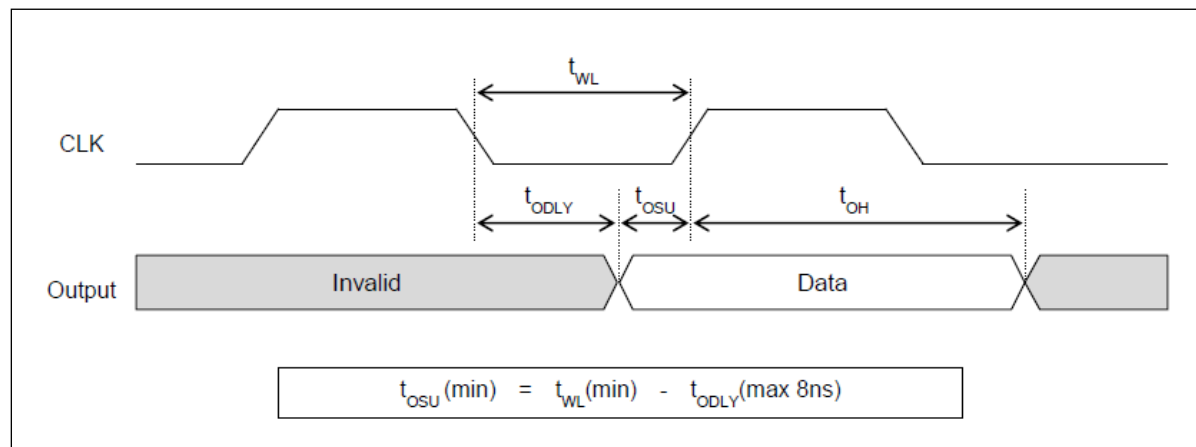
Figure 5. Output Timing Waveform
