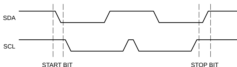
Figure 2. Start/Stop Timing
