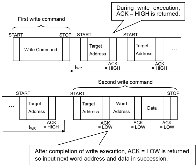
Figure 46. The Case of Continuous Write by Acknowledge Polling
