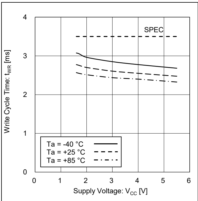
Figure 31. Write Cycle Time vs Supply Voltage
