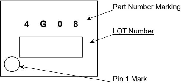
SOP-J8(TOP VIEW)
