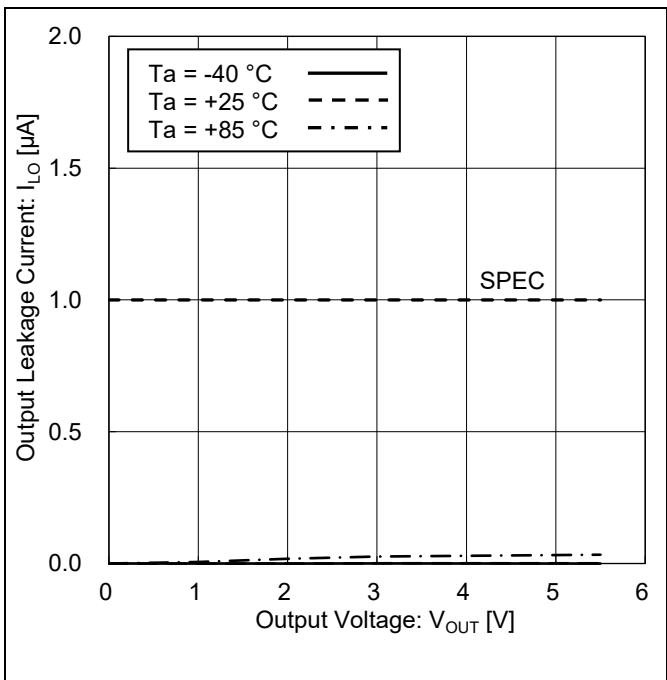
Figure 11. Output Leakage Current vs Output Voltage
