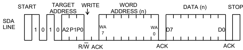
Figure 40. Byte Write
