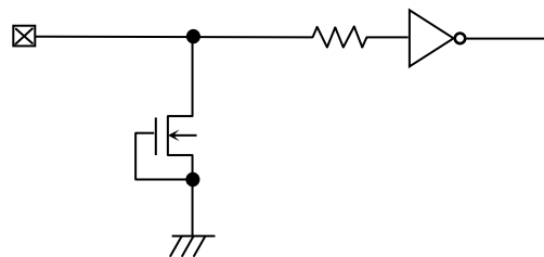
Figure 55. Input Pin Circuit Diagram (A2, WP)
