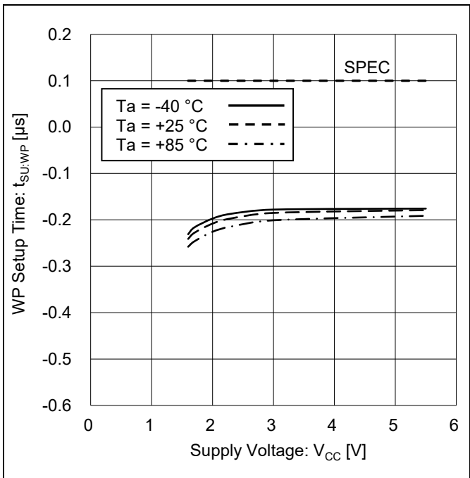
Figure 37. WP Setup Time vs Supply Voltage
