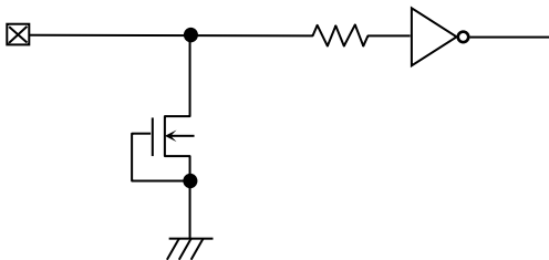
Figure 55. Input Pin Circuit Diagram (WP)
