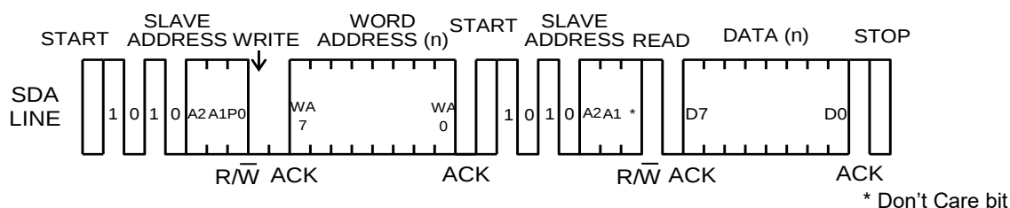
Figure 44. Random Read
