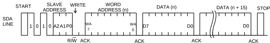
Figure 42. Page Write
