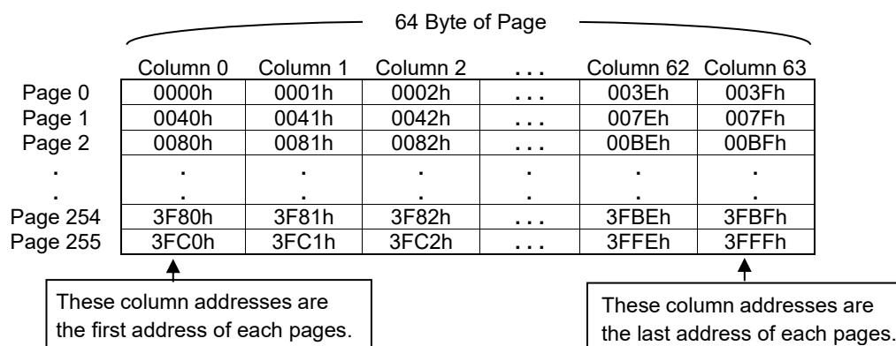
Figure 44. EEPROM physical address for Page Write command (64 Byte)
