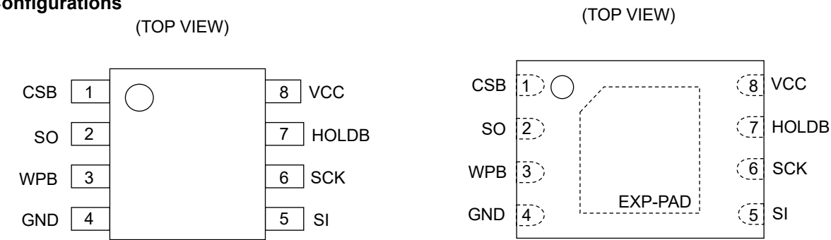
Figure 3-(a). Pin Configuration (SOP8*1, SOP-J8, TSSOP-B8, MSOP8) *1 Not Recommended for New Designs.
