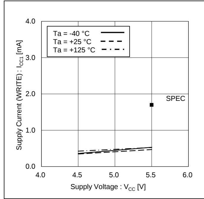
Figure 15. Supply Current (WRITE) vs Supply Voltage
