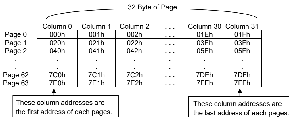
Figure 44. EEPROM physical address for Page Write command (32 Byte)
