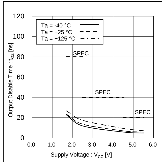
Figure 29. Output Disable Time vs Supply Voltage
