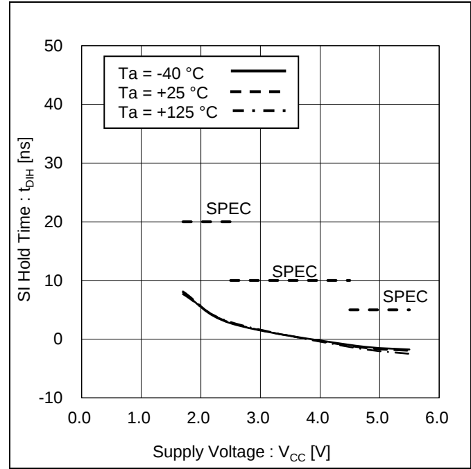
Figure 27. SI Hold Time vs Supply Voltage
