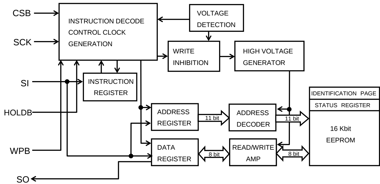
Figure 4. Block Diagram
