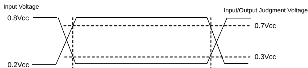
Figure 5. Input/Output Judgment Voltage
