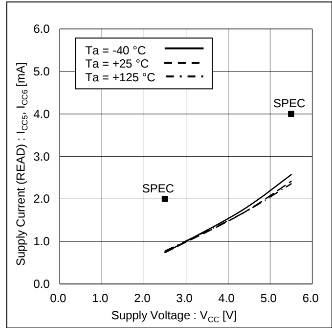
Figure 17. Supply Current (READ) vs Supply Voltage
