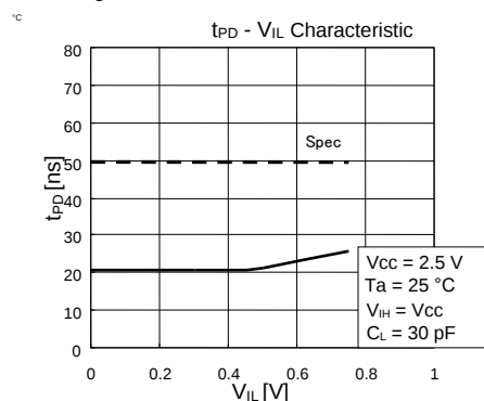
Figure 59. V_{IL} dependency of Data Output Delay Time t_{PD}
