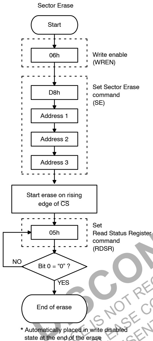
Figure 39. Sector Erase Flowcharts
